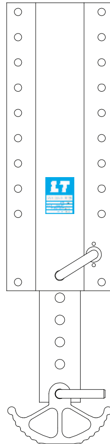
house (650mm) typeplate locking support (700 / 880 mm) handle foot
